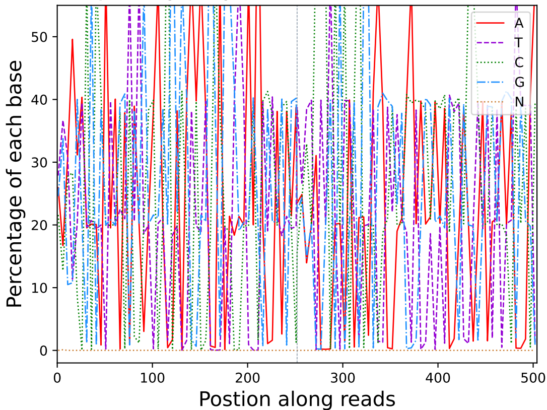
Base percentage along reads (R10125)
